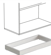
BASE FM - BS 792W x 386D x 86H
